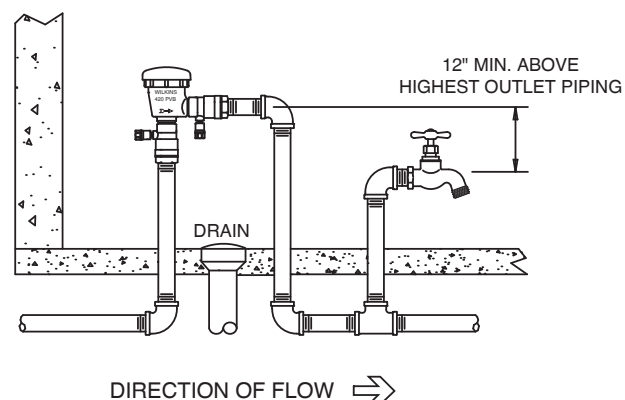
INDOOR INSTALLATION
