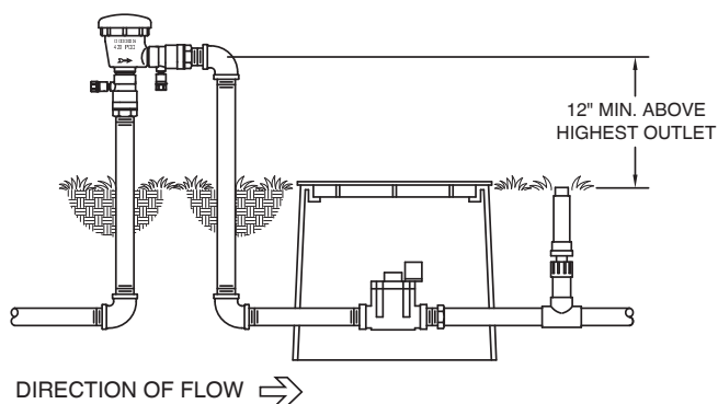
OUTDOOR INSTALLATION
